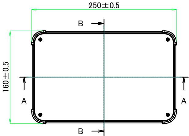
E view
